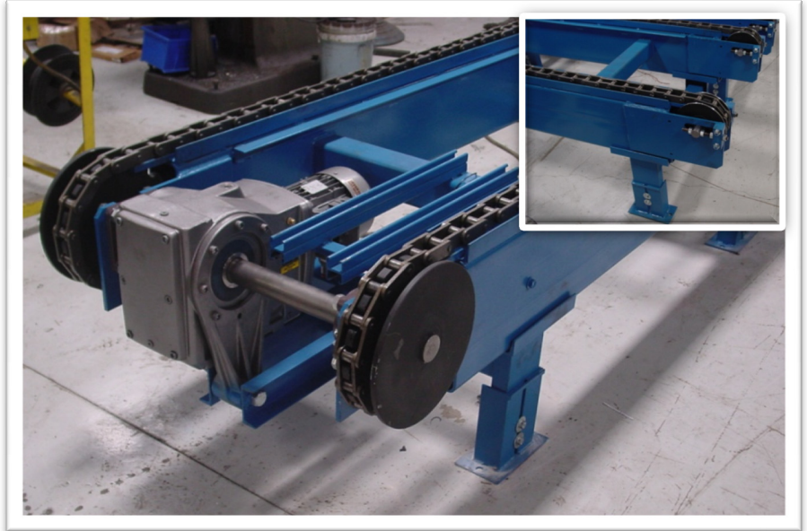
PICTURED UNITS INCLUDES SHAFT MOUNT END DRIVE, ADJUSTABLE SENSOR MOUNTS, AND OPTIONAL SPROCKET DISKS
